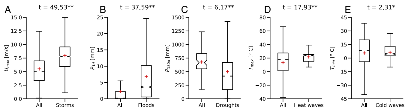
Fig. 1. Overall distributions (“All”) compared against EM-DAT-listed disaster distributions of maximum sustained wind speed at 10 m height ( U_{max} ) during storms (A), daily precipitation ( P_{1d} ) during flooding events (B), 180-d accumulated precipitation ( P_{180d} ) during droughts (C), daily maximum temperature at 2-m height ( T_{max} ) during heat waves (D), and daily minimum temperature at 2-m height ( T_{min} ) during cold waves (E). Results of Welch's t tests are included ( t -statistic); * P < 0.05 , ** P < 0.01 . Red crosses indicate mean values, notches indicate median values, and whiskers indicate quartiles.
